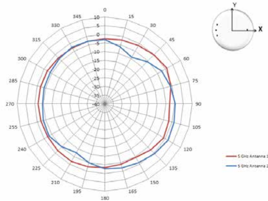
Horizontal or Azimuth (Top View)
